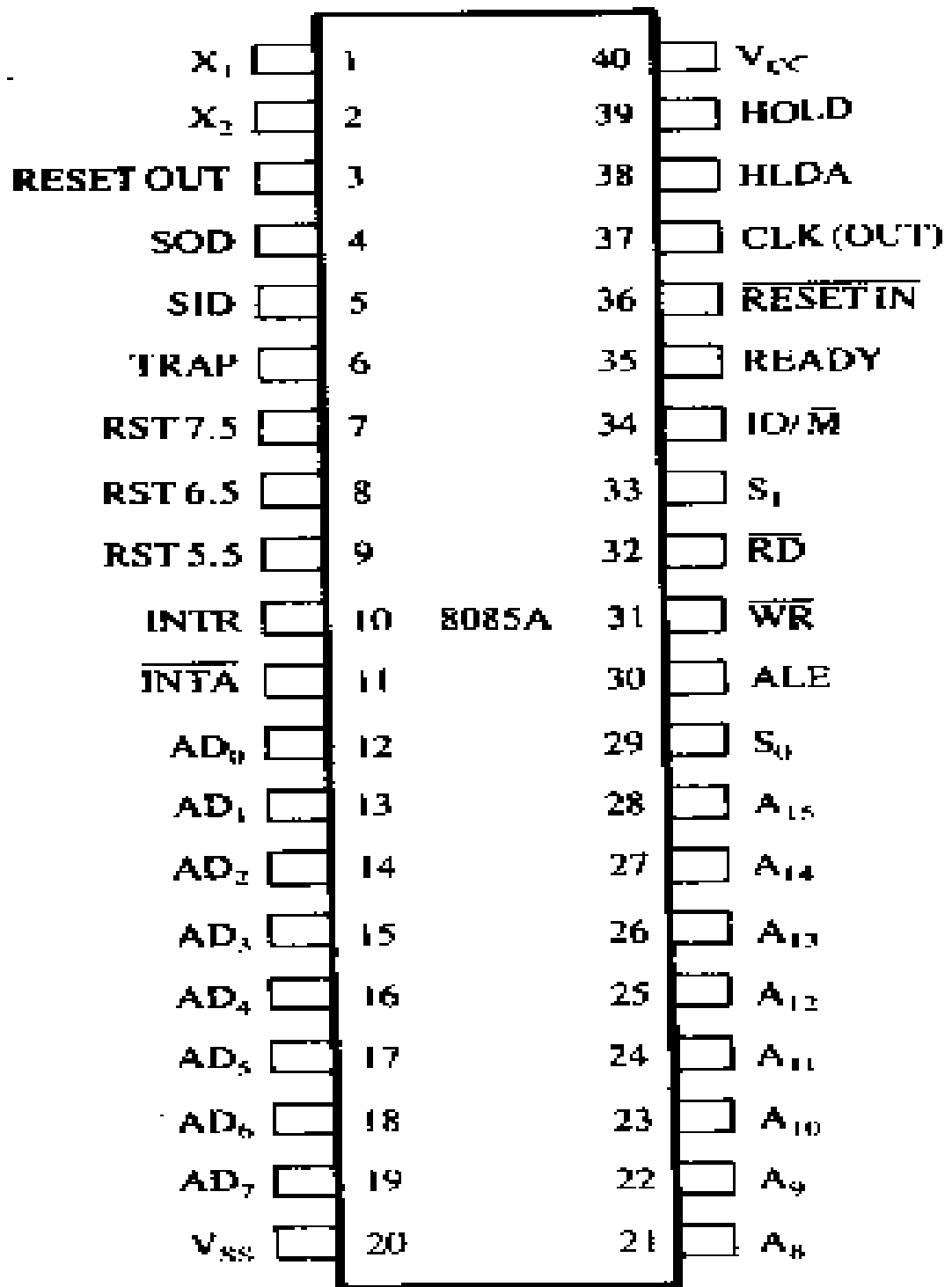
8085 Pinout
